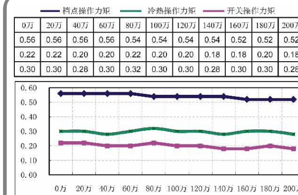
寿命测试与操作力矩图 Life test and Operation torque Curves
